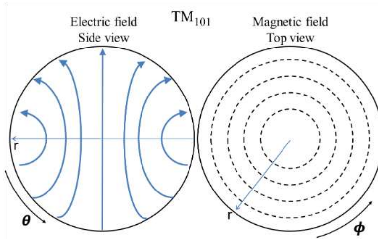
Figure 7: These cross sections of the TM_{101} mode show the orientation of its electric and magnetic fields.
