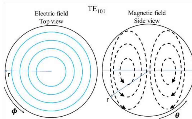
Figure 6: These cross sections of the TE_{101} mode show the orientation of its electric and magnetic fields.
