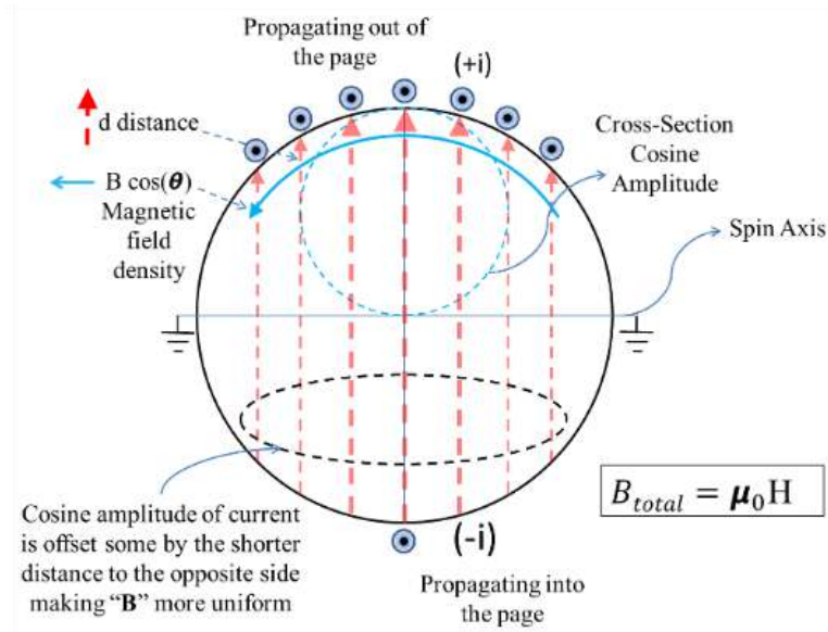
Figure 14: The strength of the magnetic field density B at the opposite point on the surface of the sphere is fairly uniform like that of a planar current sheet.
