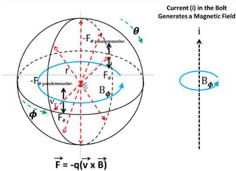
Figure 5: The Force on the expanding electron cloud due to the current of the lightning bolt causes the electrons to rotate around the charge center in the direction of theta.
