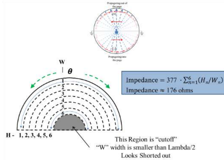
Figure 9: TEM wave-front impedance calculation. There is a fixed amount of energy, charge, and therefore voltage in the expanding volume. The electric and magnetic fields are related by the free space impedance of 377 ohms per unit area.
