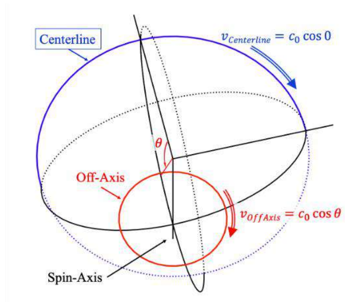
Figure 10: A plane wave propagating around its spin axis has a wave velocity that is a function of theta ( \theta ). Theta is the angle between the wave centerline and any off-axis component.
