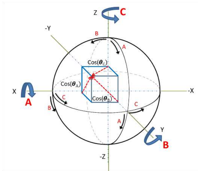
Figure 15: The Force each wave provides at any point on the sphere is proportional to the cosine 2 of the off-axis angle of its plane wave. Consequently, the total force from the three tori pushing inward on the surface of the sphere is uniform.
