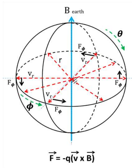
Figure 4: The force on the expanding electron cloud due to the earth's magnetic field causes the electrons to rotate around the charge center in the direction of \Phi(\phi) .
